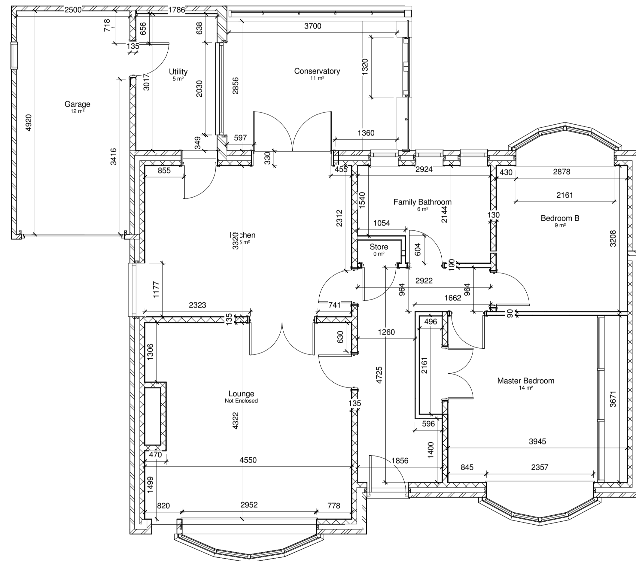
1 L0 - Ground Floor Existing 1 : 50
